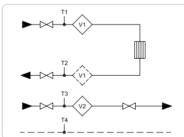
Example 2: Closed thermal system with 2 flow meters
